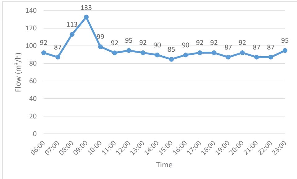
Figure 50: Variation of inflow at STP
