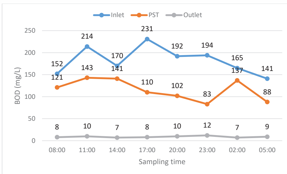
Figure 21: BOD variation at STP
