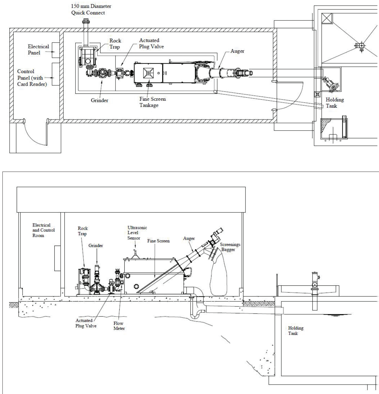
Figure 65: Typical plan and elevation of a septic receiving station
