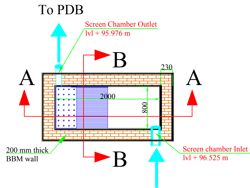
Plan of Screen Chamber
