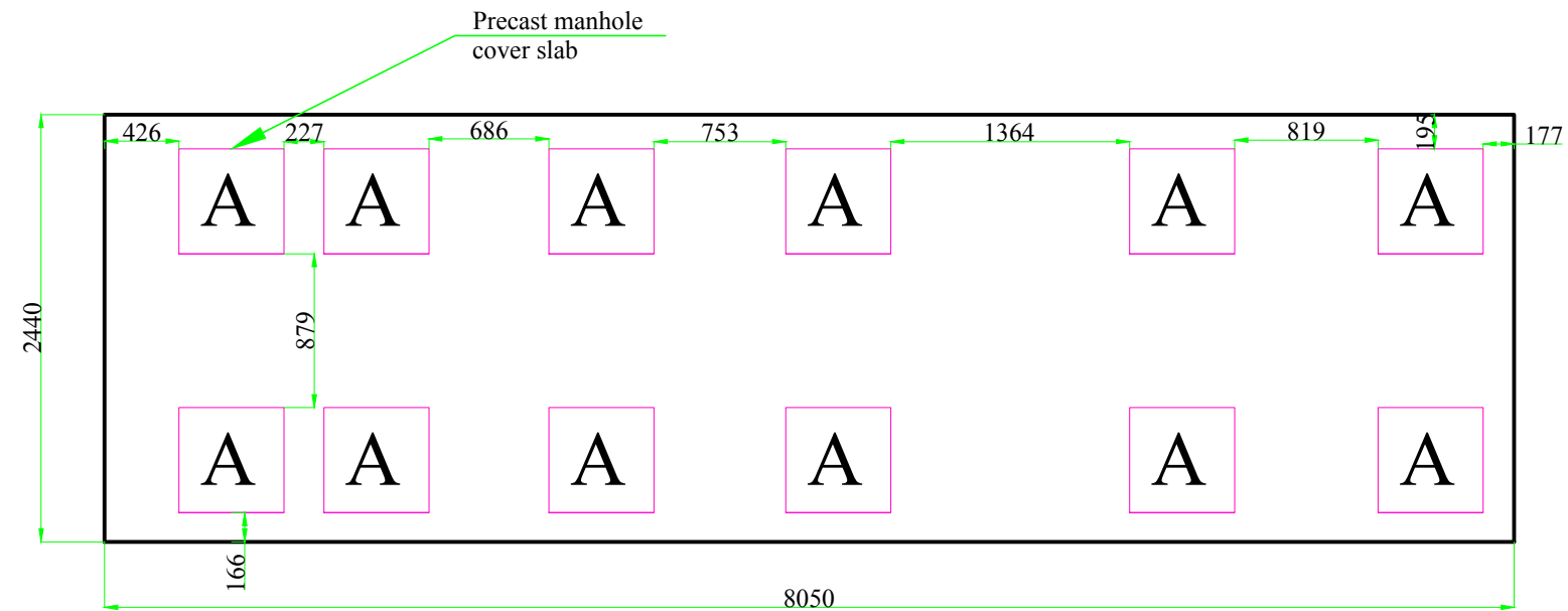
Plan of Manhole
