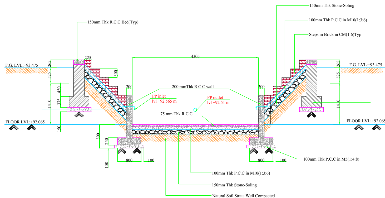
Cross Section of A-A
