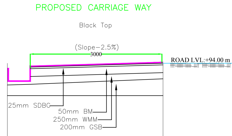
TYPICAL CROSS SECTION OF BLACKTOP ROAD
