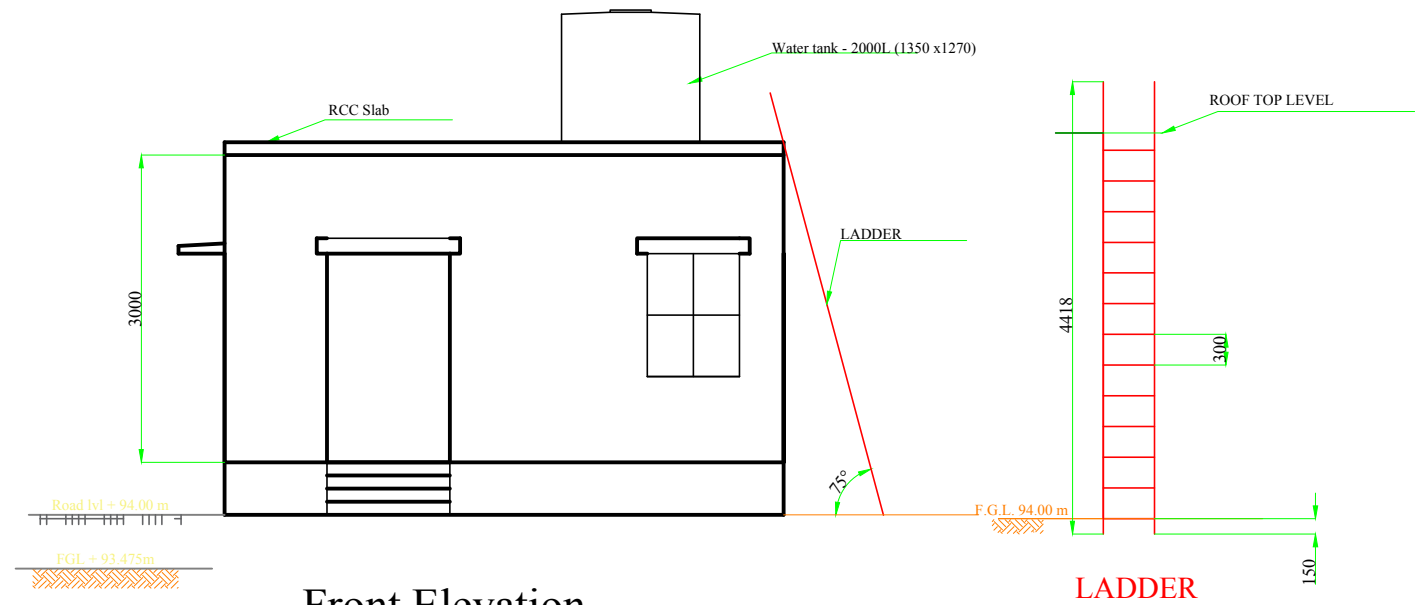
Front Elevation
