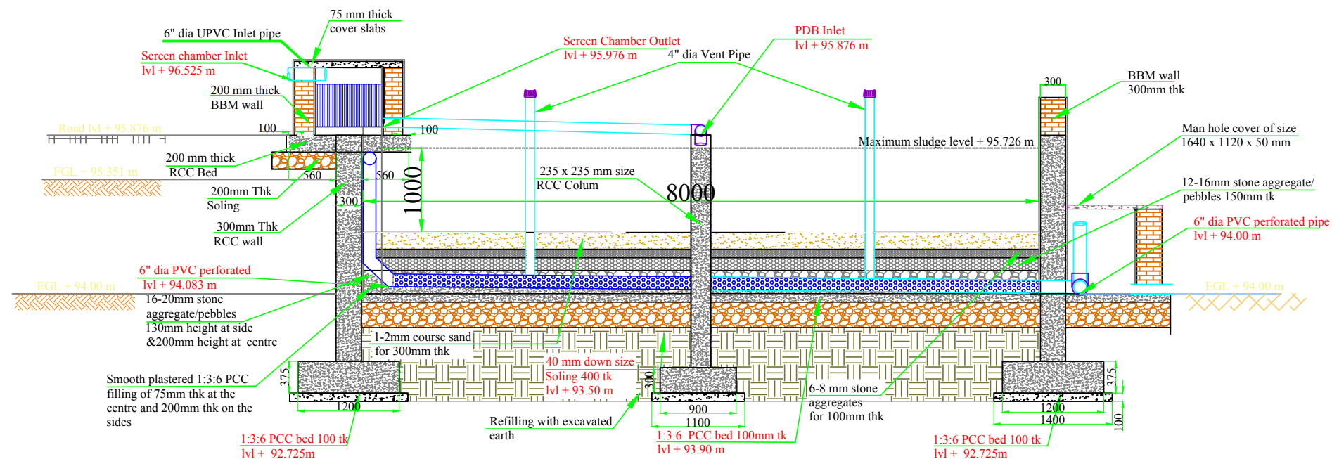
Cross Section of B-B
