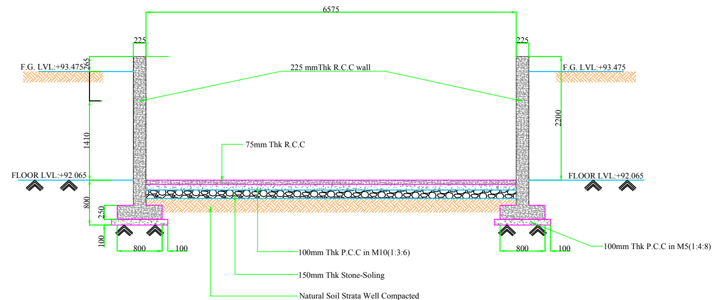
Cross Section of B-B
