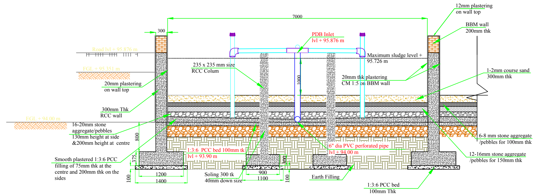
Cross Section of A-A
