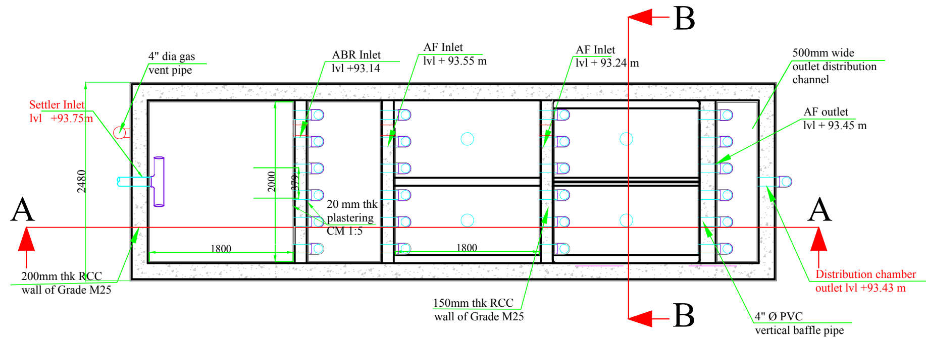
Plan of Integrated Settler and Anaerobic Filters
