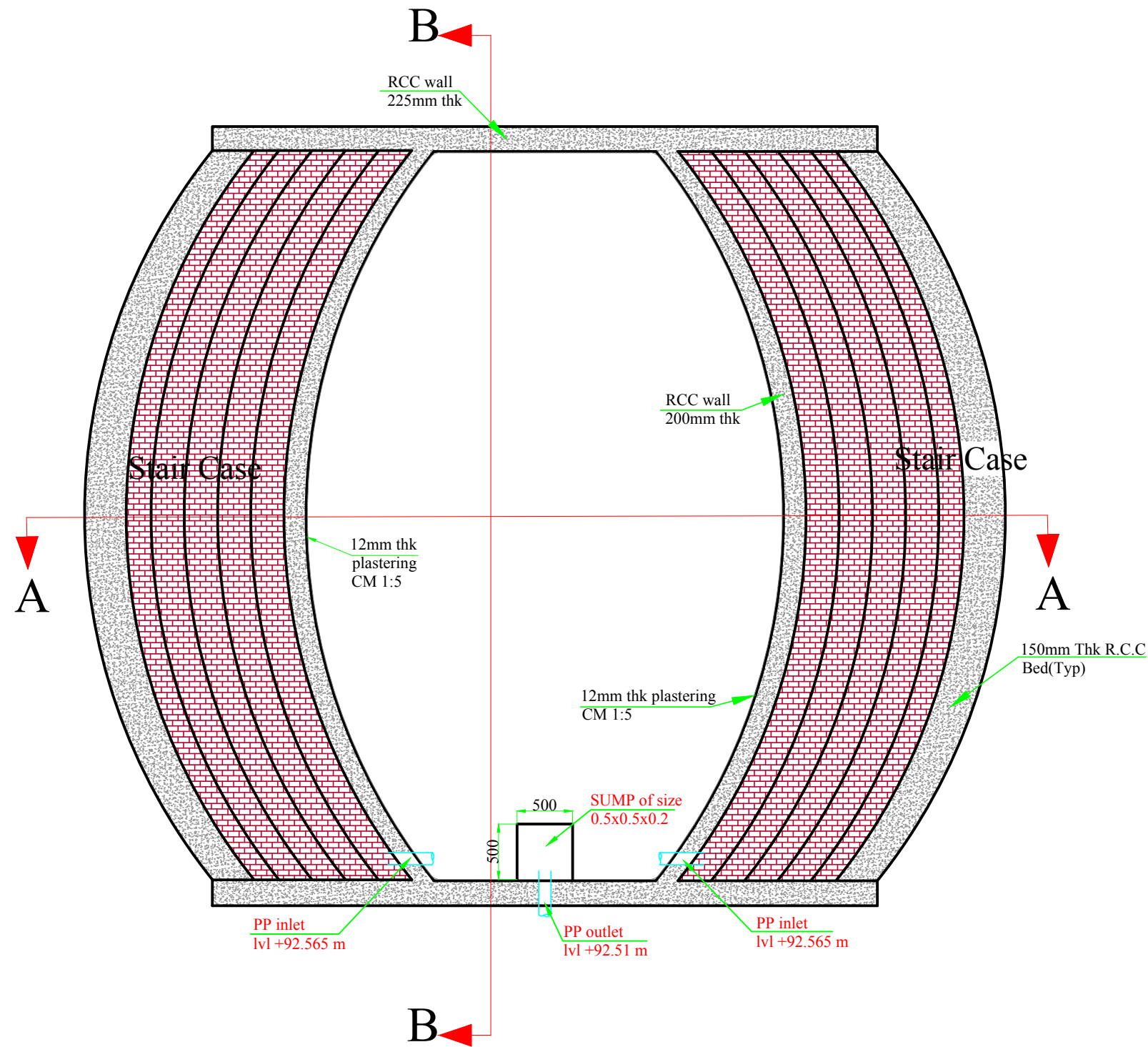
Plan of Polishing Pond
