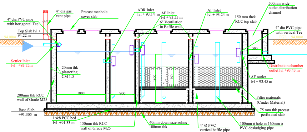
Integrated Settler and Anaerobic Filters
