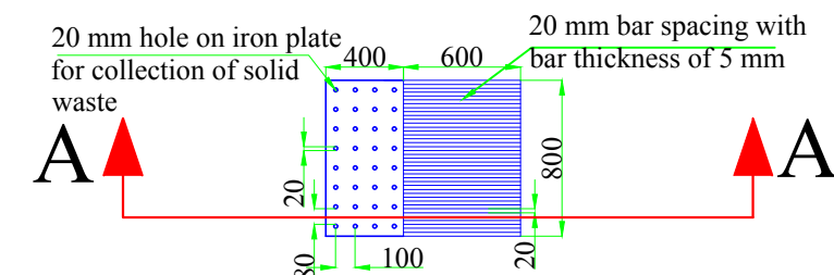
Screen Bar Details
