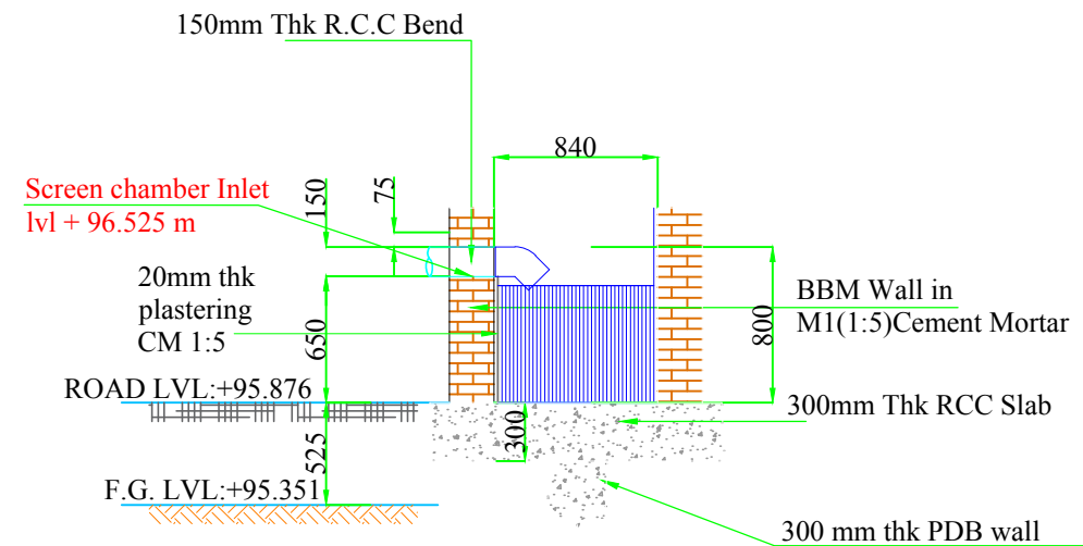
Cross Section of B-B
