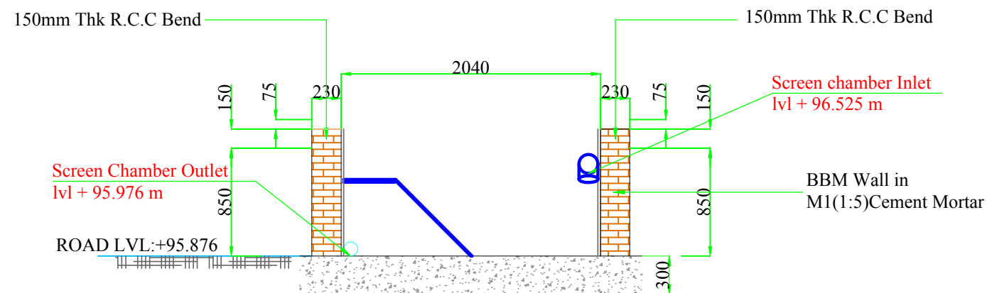
Cross Section of A-A
