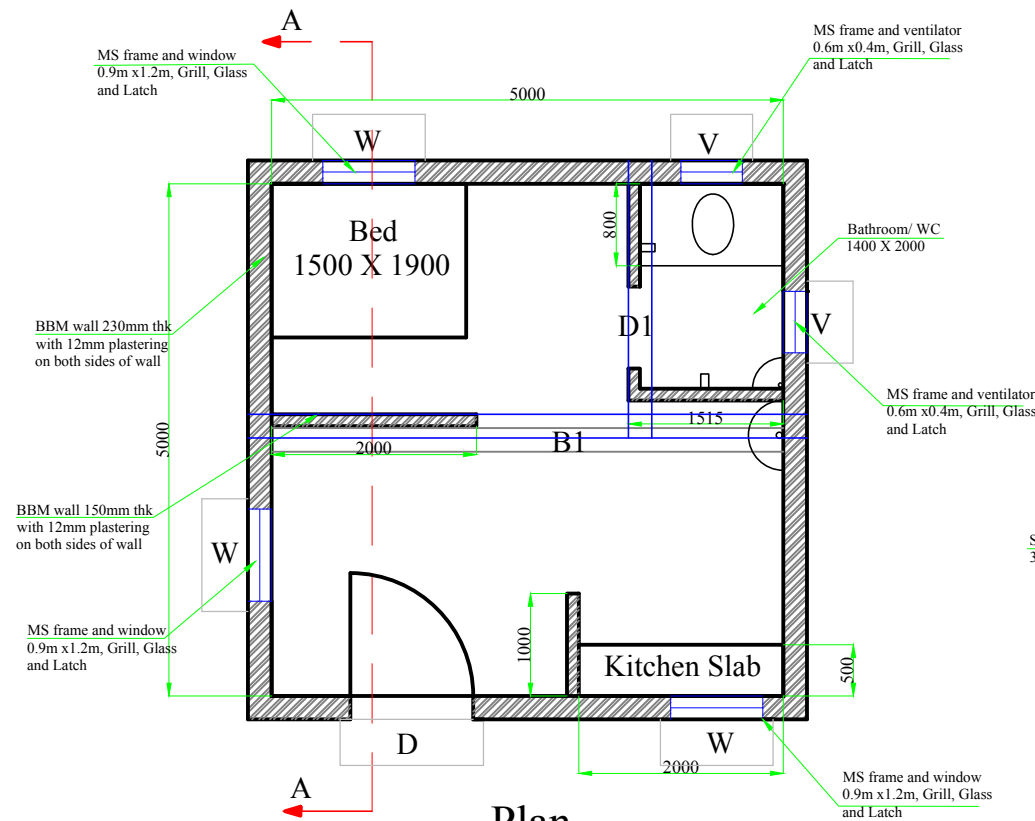
Plan
