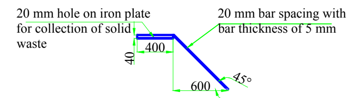
Screen cross section A-A
