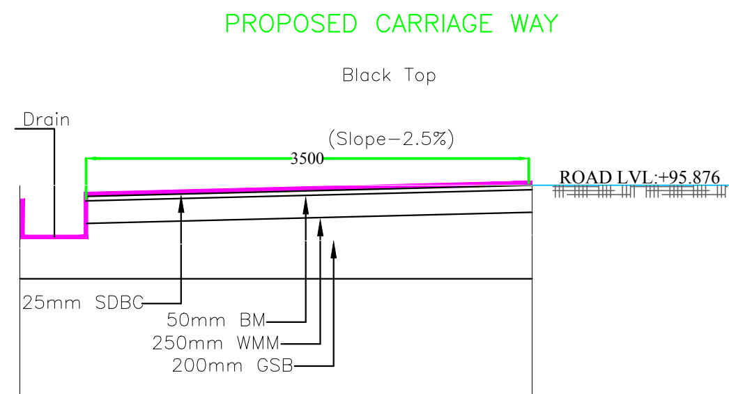
TYPICAL CROSS SECTION OF BLACKTOP ROAD
